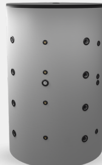
Buffer tank 2000 L, two heat exchangers, non-enameled
